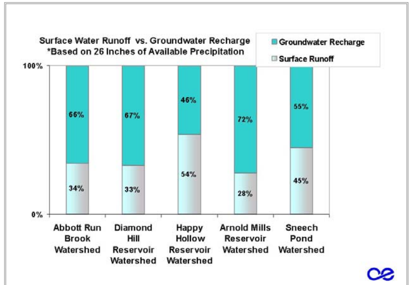
Figure 6b. Water Budgets
