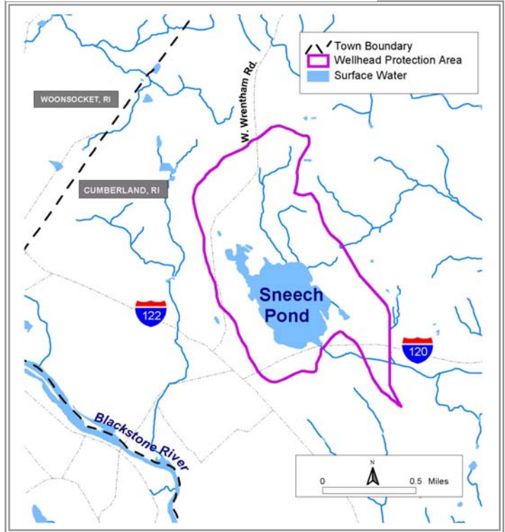
Map 6: Sneeched Pond Watershed
