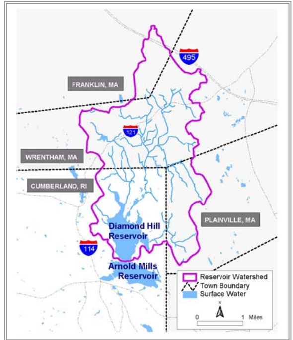
Map 2: Diamond Hill Reservoir Watershed
