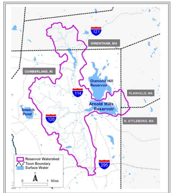
Map 3: Arnold Mills Reservoir Watershed
