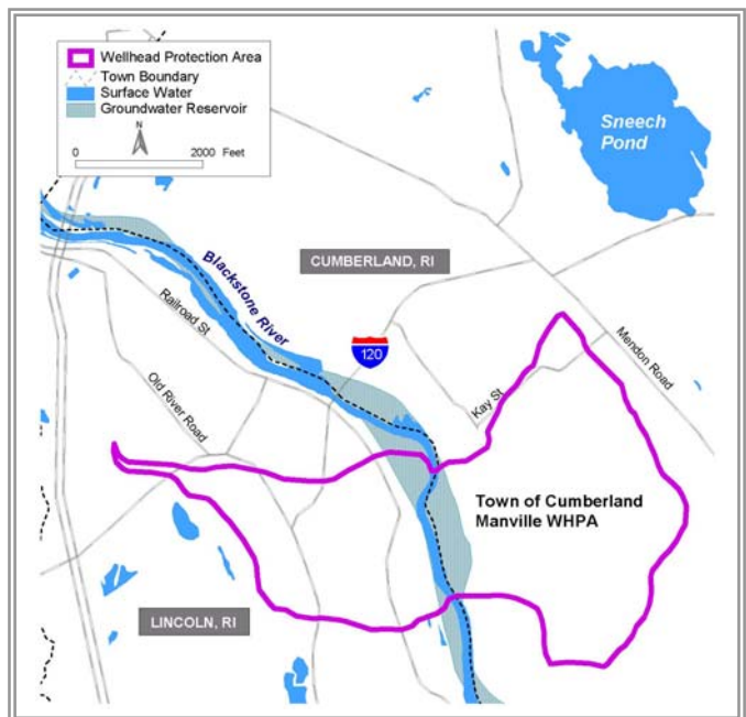
Map 9: The Manville WHPA
