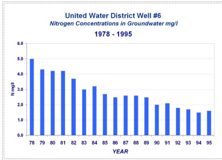
Figure 1. Nitrogen Concentrations in United Well #6, 1978 – 1995 (Source: RI HEALTH Water Quality Monitoring Data)
