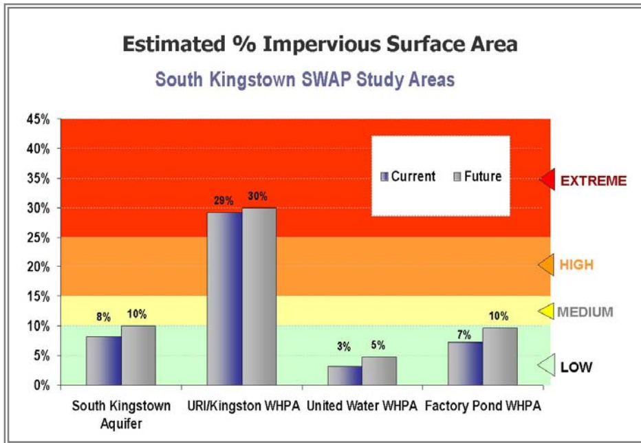
Figure 4. Estimated Impervious
