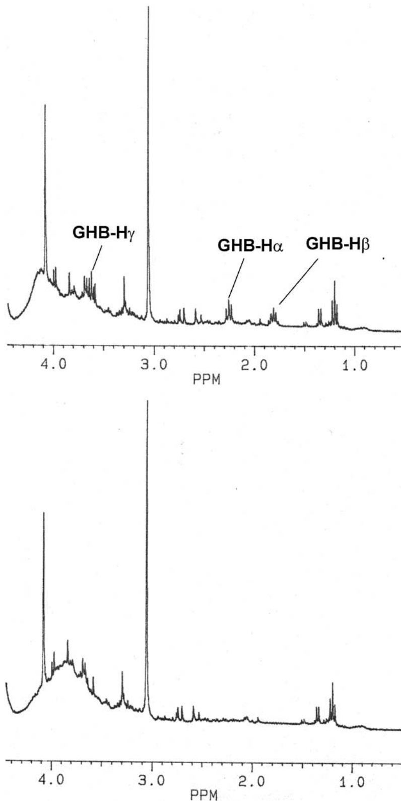
FIG. 4—Typical 1 H NMR spectra of GHB (0.2 mg/mL) in urine (upper trace) and negative control (lower trace).
